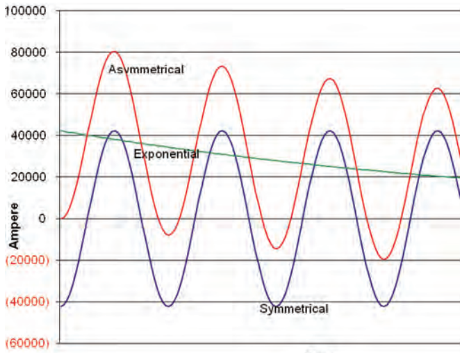
Asymmetrical Current (30 kA, X/R=30) Figure B-1
