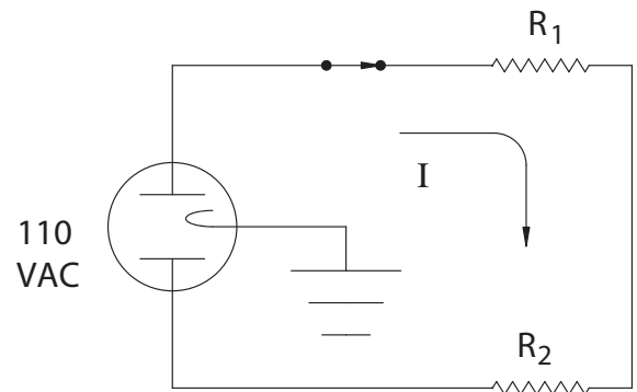
Series Circuit Using Common Symbols Fig. 5-3
