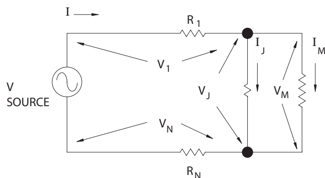
Voltage Division Using the Neutral Fig. 7-1
