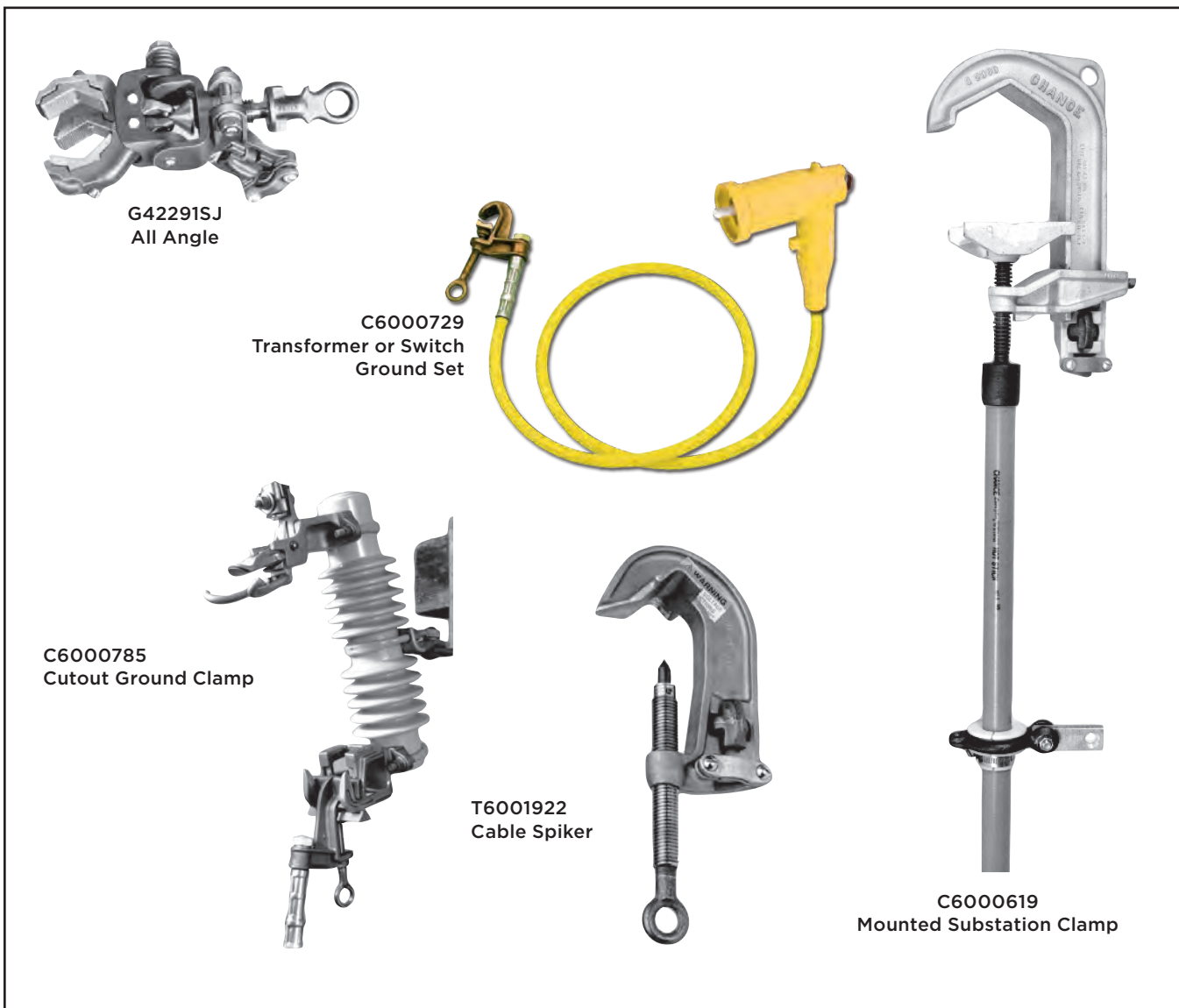
Special Purpose Clamps Figure 8-6
