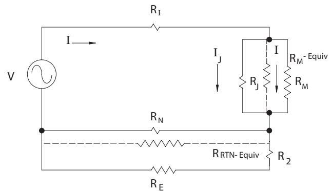
Series/Parallel Circuit Fig. 5-8
