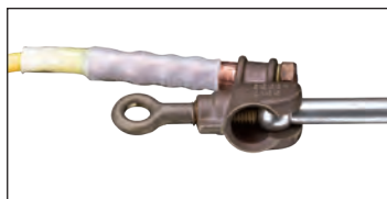
*Long Ball Stud T6002364 3" nominal shank length Weight, each: 3/4 lb. / 0.3 kg. 5/8" dia. shank
